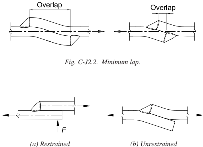
Fig. C-J2.3. Restraint of lap joints.
