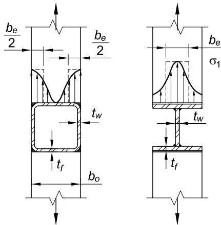
Fig. C-K1.3. Elastic uneven stress distributions in HSS and wide-flange members.
