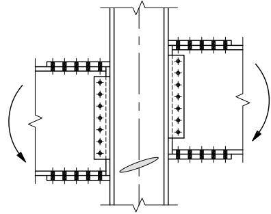
(b) Offset back-to-back moment connections under gravity load, Section J10.5 applies
