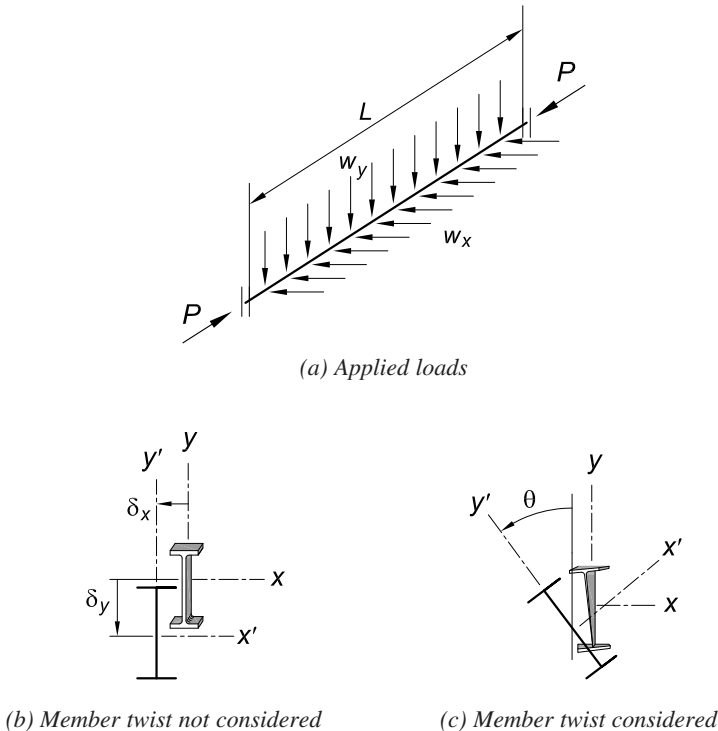
Fig. C-A-1.1. Deflection of cross section at midspan.
