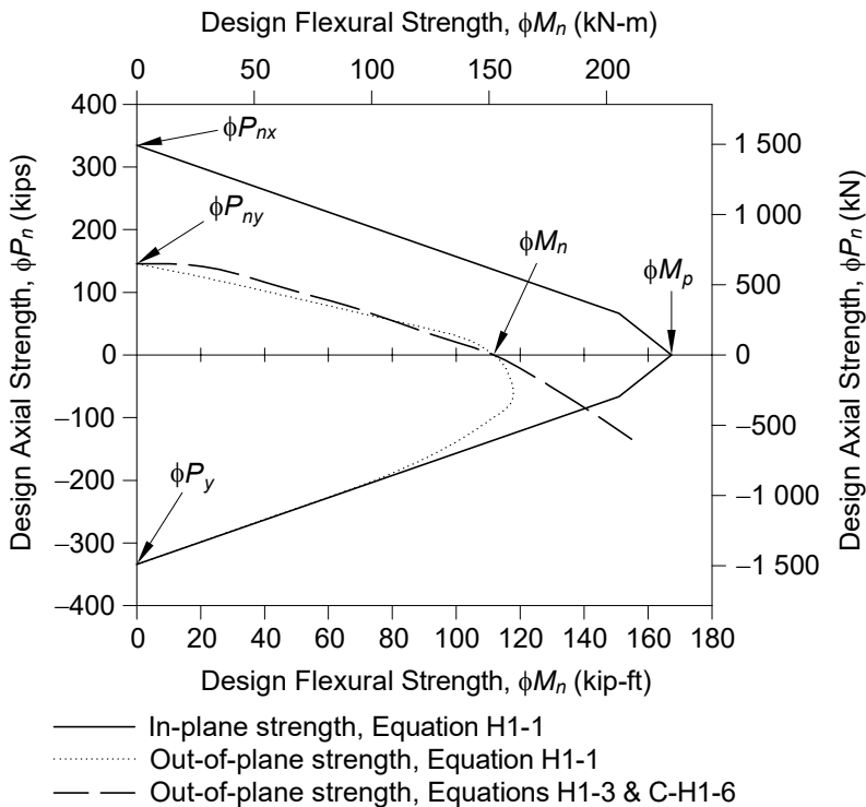
Fig. C-H1.5. Beam-columns under compressive and tensile axial force (tension is shown as negative) (LRFD) (W16×26, F_y = 50 ksi, L_b = 10 ft, C_b = 1 ) (W410×38.8, F_y = 345 MPa, L_b = 3.1 m, C_b = 1 ).
